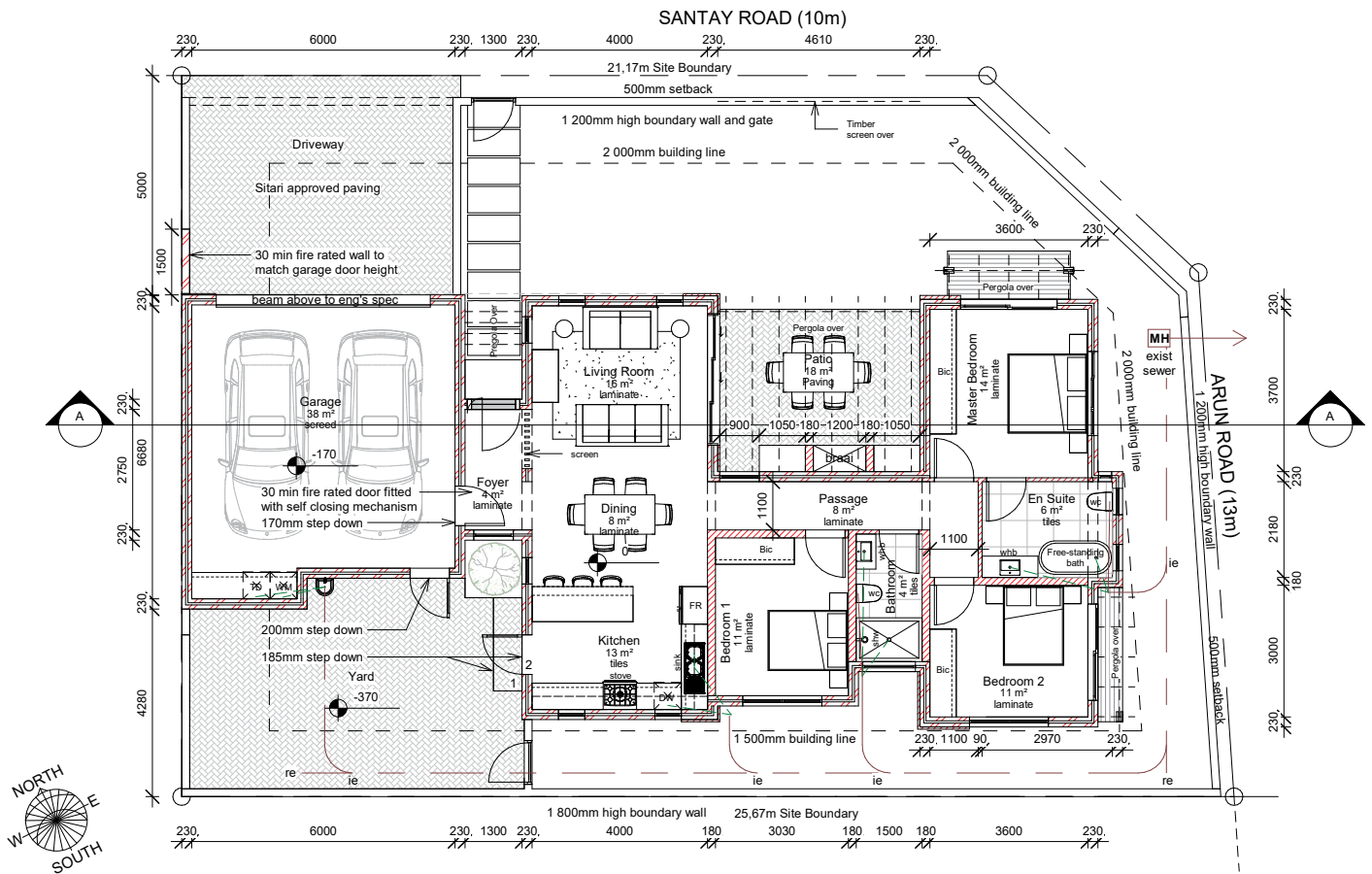
GROUND FLOOR STOREY 1:100
